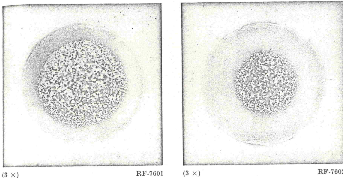
Fig. 1. Photomicrographs of cross-sections from the middle of rods 20 (on left) and 21 (on right). These illustrate the quenching effect of a cool extrusion container on the thickness of the fine-grained rim. Rod 21 was the rear billet in a tandem extrusion and was in contact with the cool extrusion container (250° C) for 3 sec longer than rod 20.
